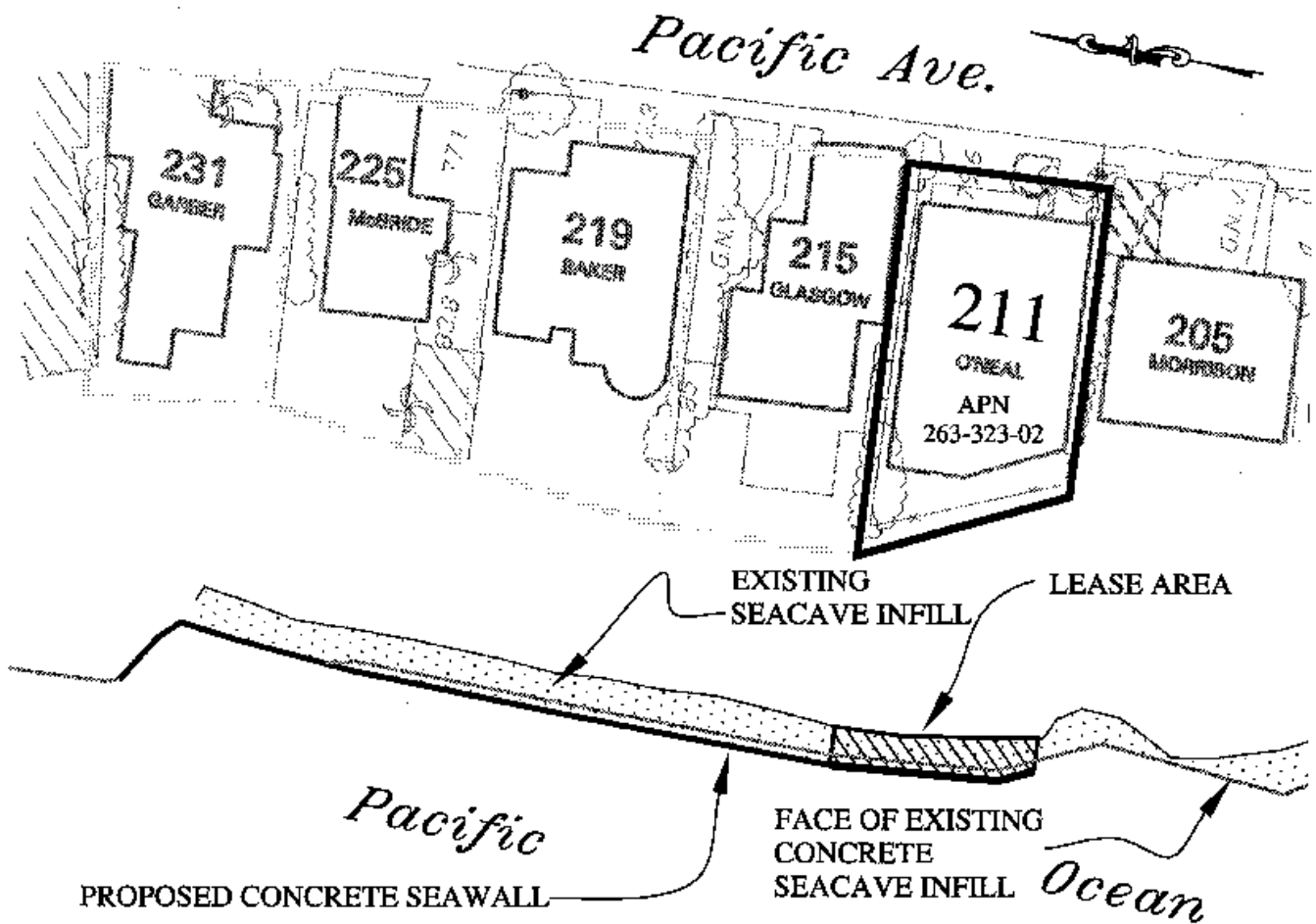
211 PACIFIC AVENUE, SOLANA BEACH PROPOSED SEAWALL AND EXISTING SEA CAVE INFILL
