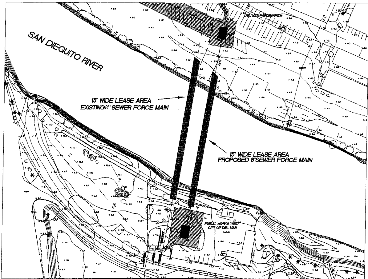
PROPOSED 8" SEWER FORCE MAIN AND EXISTING 8" SEWER FORCE MAIN
