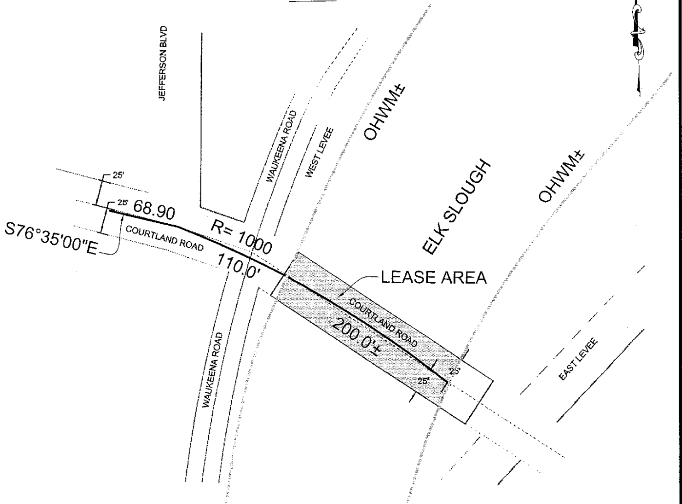
BRIDGE CROSSING, ELK SLOUGH, COUNTY ROAD 158 (COURTLAND ROAD)
