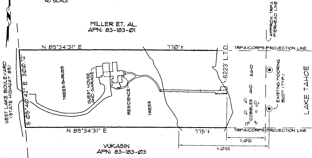
BUOY DETAIL NO SCALE
