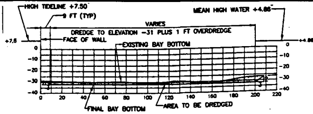
TYPICAL SECTION SCALE: 1" = 60'
