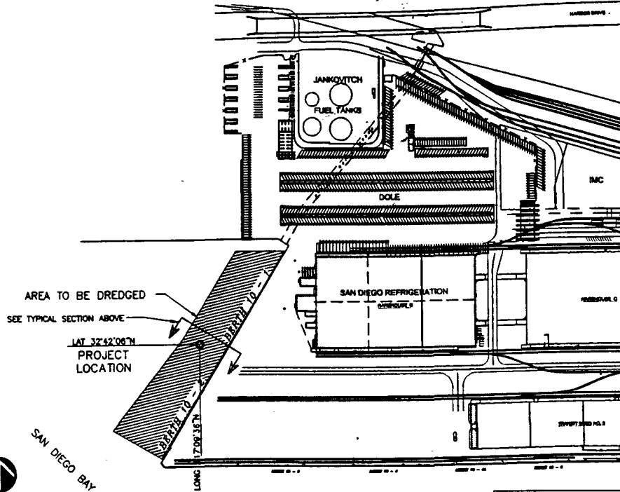
SITE PLAN SCALE: 1" = 400'
