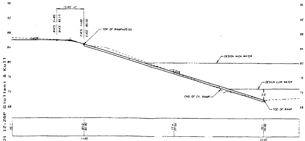
PROFILE - BOAT RAMP SCALE H:V = 10:1
