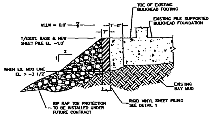
SECTION AT SHEET PILE: CASE III
