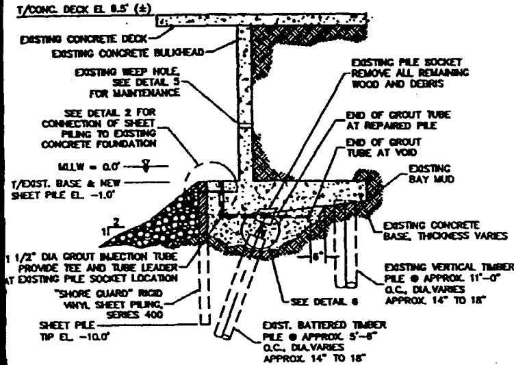
SECTION AT TIMBER PILE REPAIR
