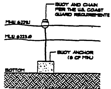
BUOY DETAIL NO SCALE
