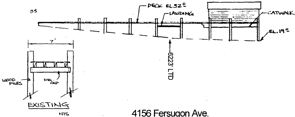
PLAN + PROFILE
