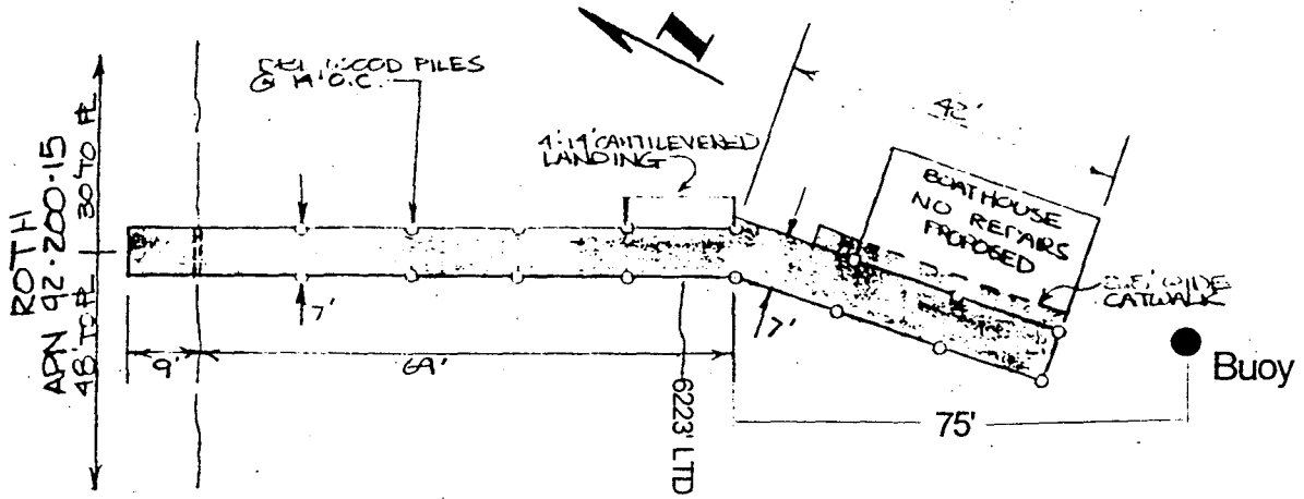
PLAN + PROFILE
