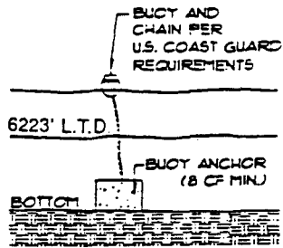
BUOY DETAIL
