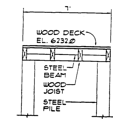
EXISTING PIER WALKWAY NO SCALE
