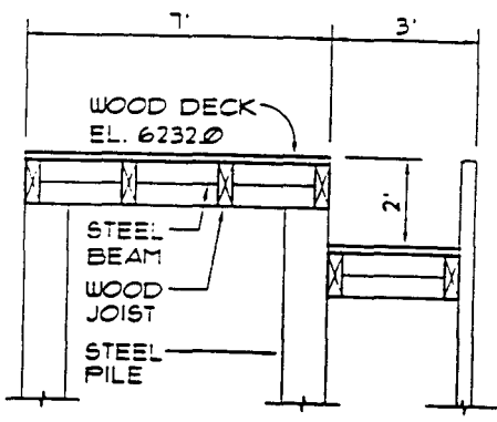
TYPICAL PIERHEAD SECTION NO SCALE
