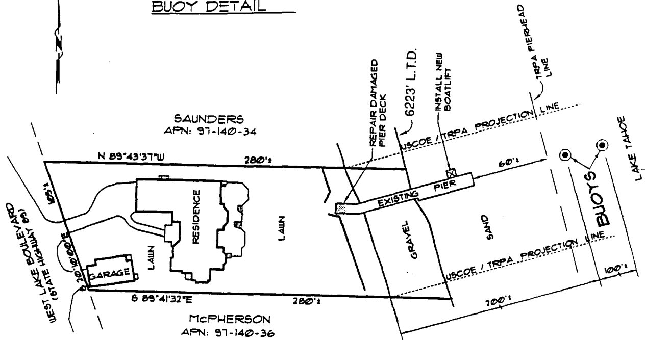
BUOY DETAIL
