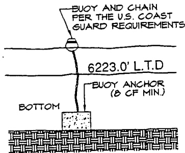
BUOY DETAIL NO SCALE
