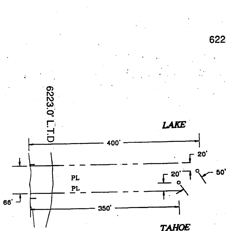
BUOY PLAN
