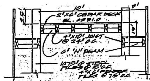
PIERHEAD SECTION
