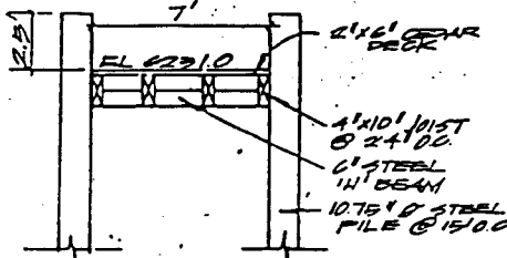
WALKWAY SECTION
