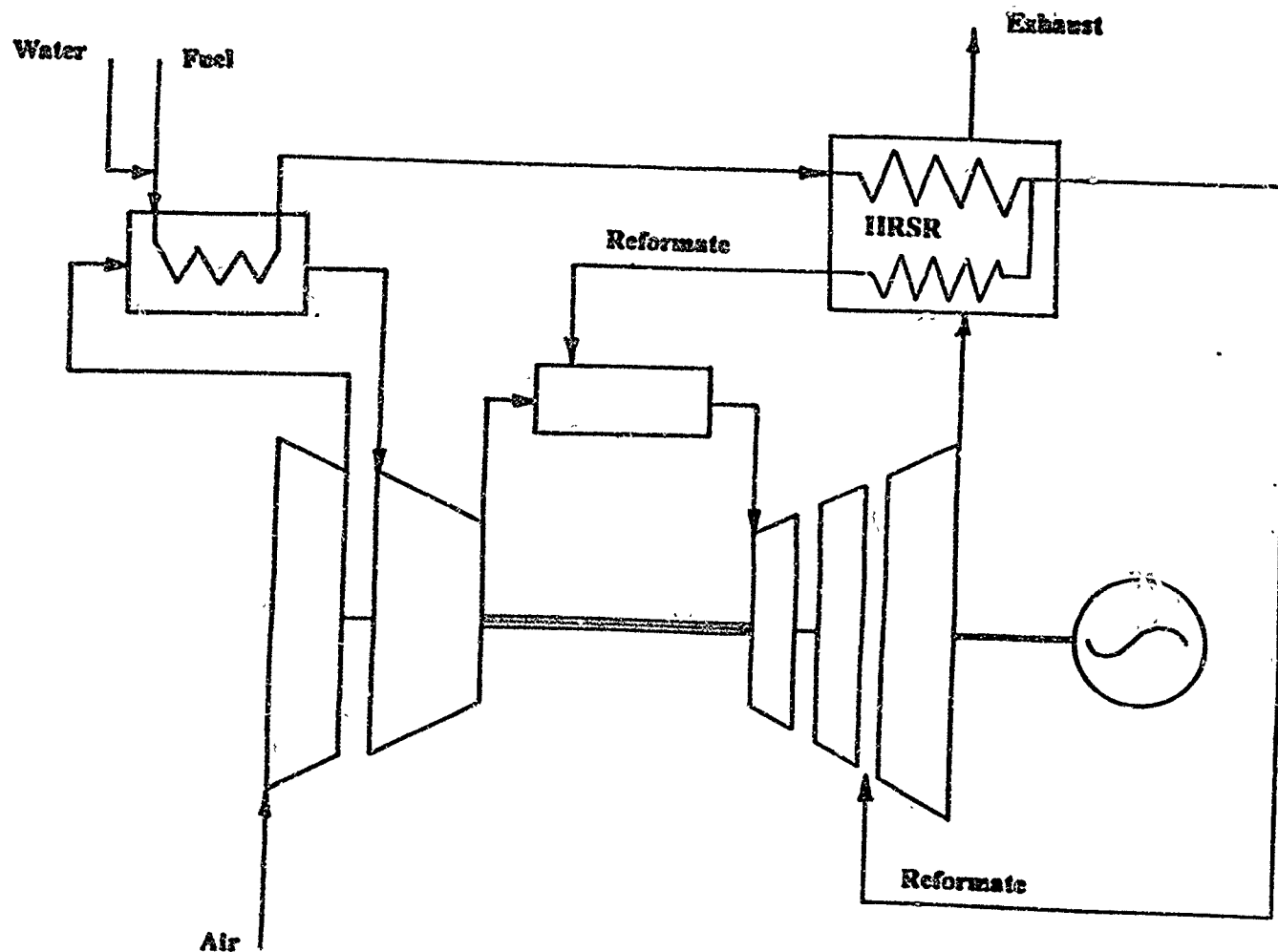
IR-CRGT (Intercooled Reheat Chemically Recuperated Gas Turbine)
